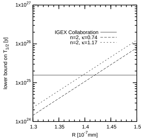
FIG. 1. Lower bounds on the half-life of neutrinoless double beta decay in the case of two additional spatial dimensions of size R . The mass of the messenger particle is m_\chi = 10 keV.
